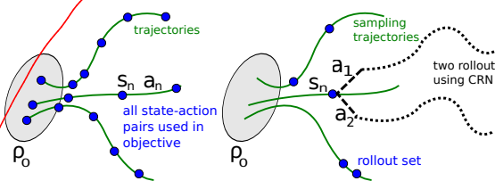
Figure 1. Left: illustration of single path procedure. Here, we generate a set of trajectories via simulation of the policy and incorporate all state-action pairs (s_n, a_n) into the objective. Right: illustration of vine procedure. We generate a set of “trunk” trajectories, and then generate “branch” rollouts from a subset of the reached states. For each of these states s_n , we perform multiple actions ( a_1 and a_2 here) and perform a rollout after each action, using common random numbers (CRN) to reduce the variance.
